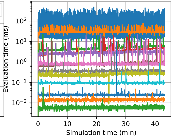
Process.calculateRequest
