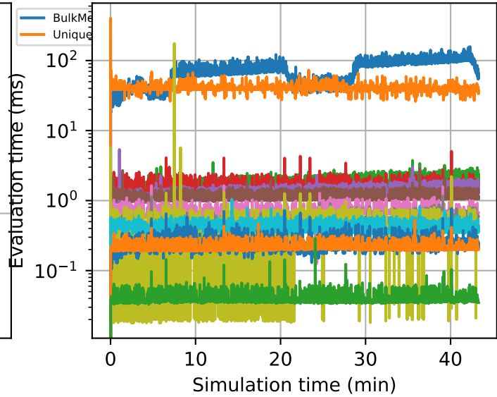
Process.evolveState
