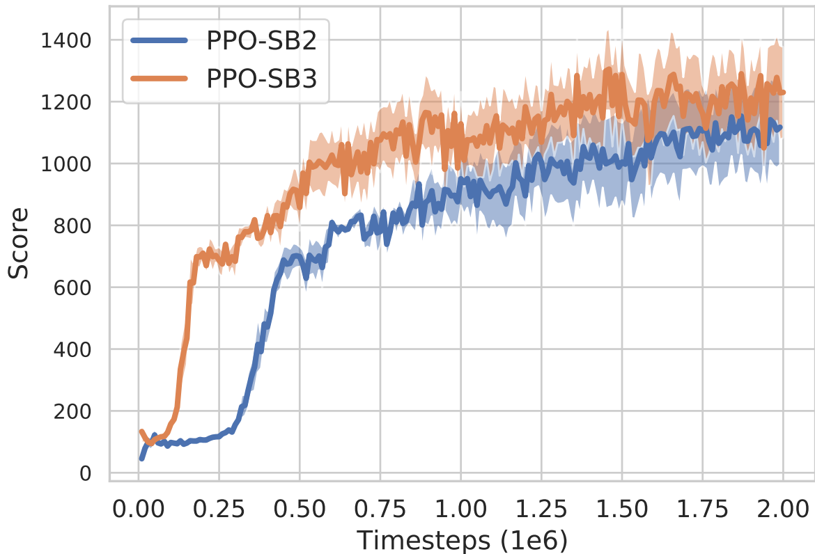
Walker2DBulletEnv-v0
