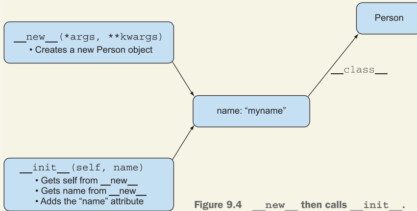
Figure 9.4 __new__ then calls __init__ .
