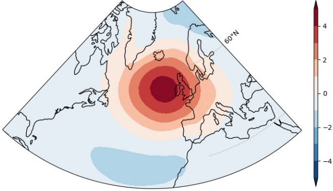
NAO: CMIP6 MPI-ESM1-2-LR (r1i1p1f1) - EOF2 1850-2849 JFM 15.0%
