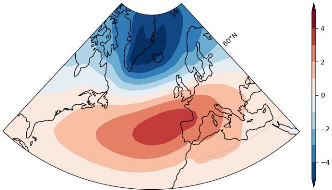
NAO: CMIP6 MPI-ESM1-2-LR (r1i1p1f1) - EOF1 1850-2849 JFM 45.8%
