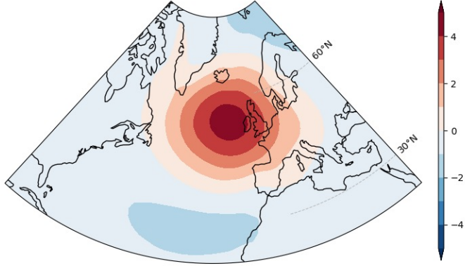
NAO: CMIP6 MPI-ESM1-2-LR (r1i1p1f1) - EOF2 1850-2849 JFM 15.1%
