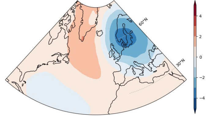
NAO: CMIP6 MPI-ESM1-2-LR (r1i1p1f1) - EOF3 1850-2849 JFM 12.0%
