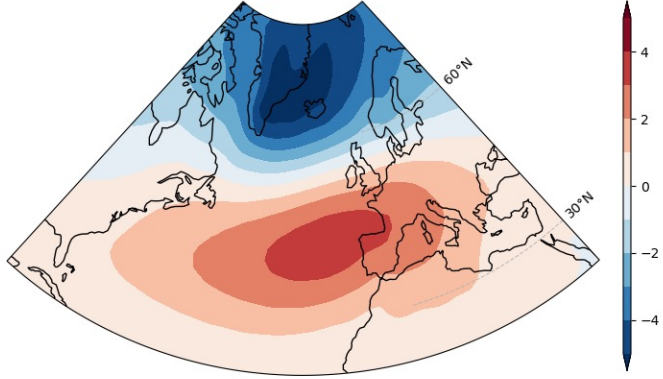
NAO: CMIP6 MPI-ESM1-2-LR (r1i1p1f1) - EOF1 1850-2849 JFM 45.7%
