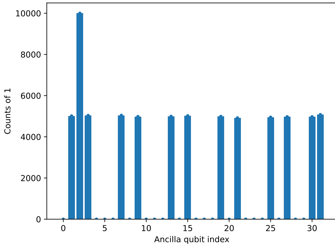
Measure all ancilla
