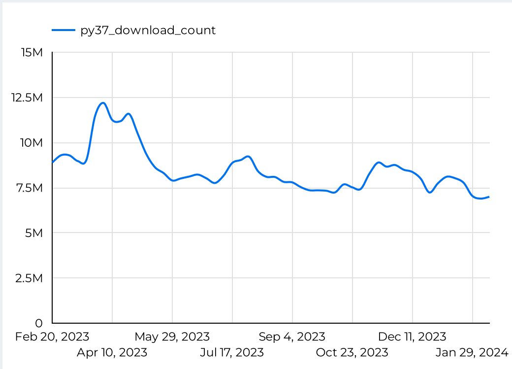
Python 3.7 downloads
