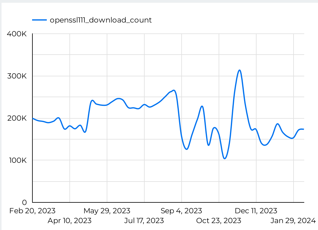
OpenSSL 1.1.1 downloads
