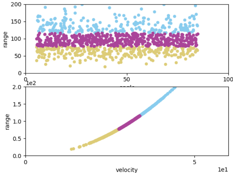
Figure 32. K-means clustering on projected parameters.
