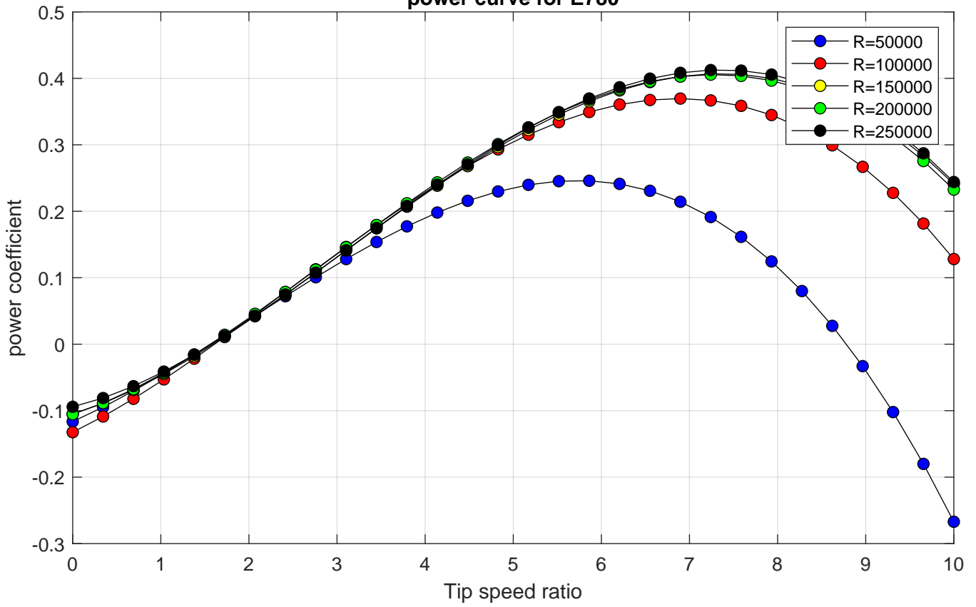
power curve for E780
