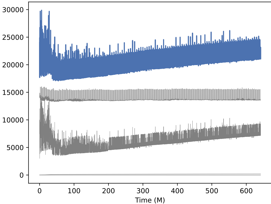
Total Memory Usage (MB)
