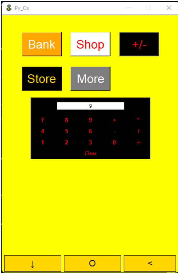
Calculator App
