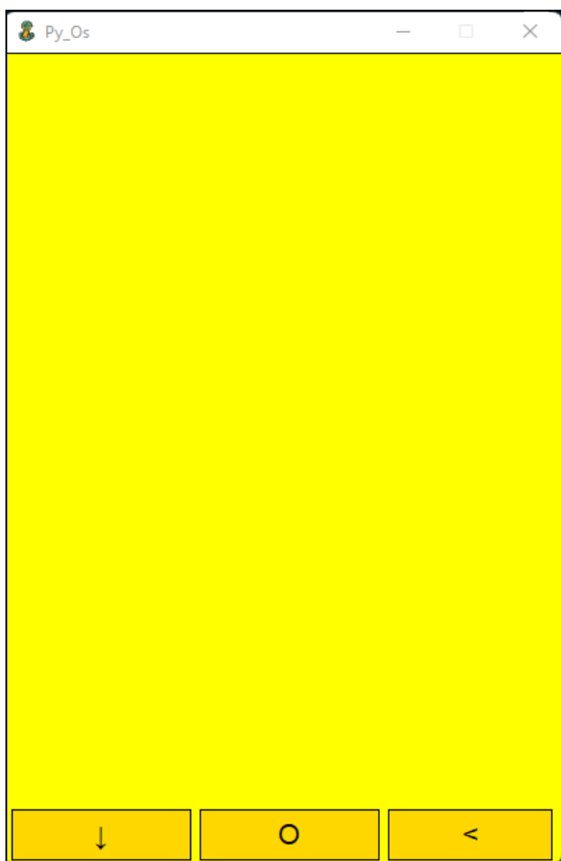
Main Window
