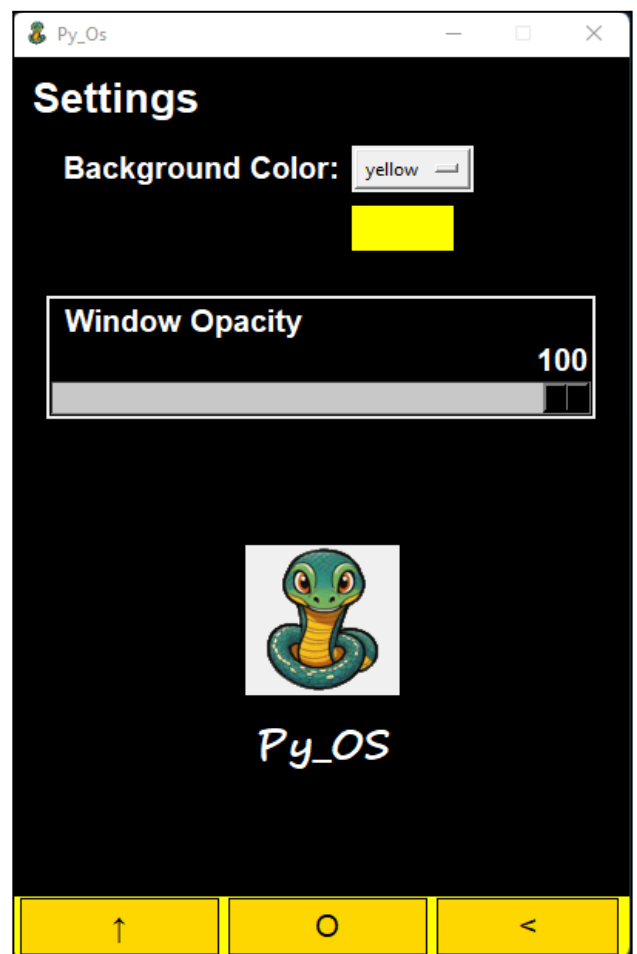
Customization/Settings
