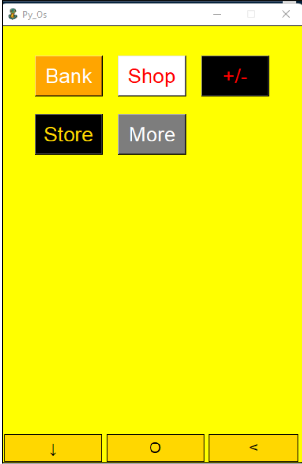
App Drawer
