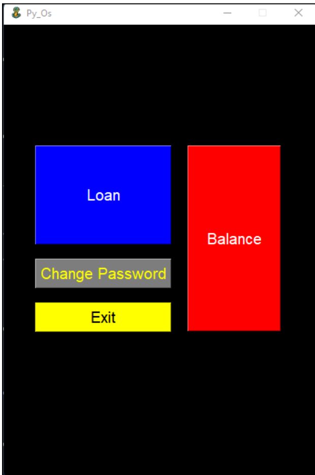
App Drawer
