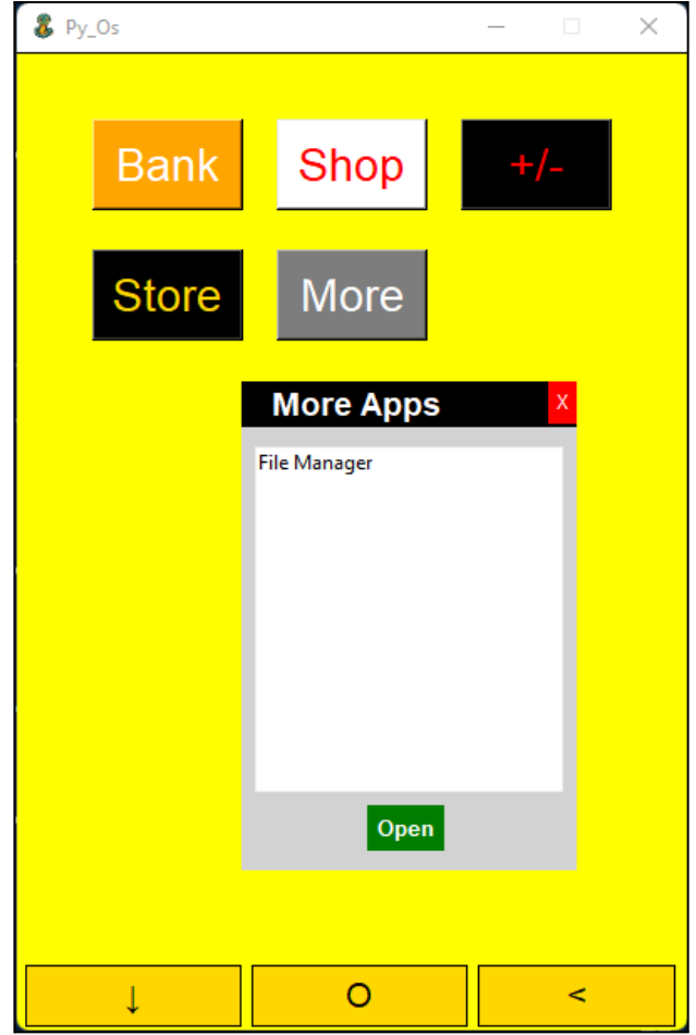
More Apps
