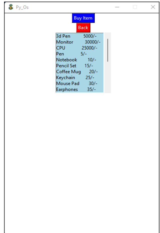
More Apps
